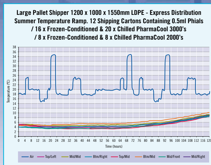
Large Pallet Shipper +2°C to +8°C
