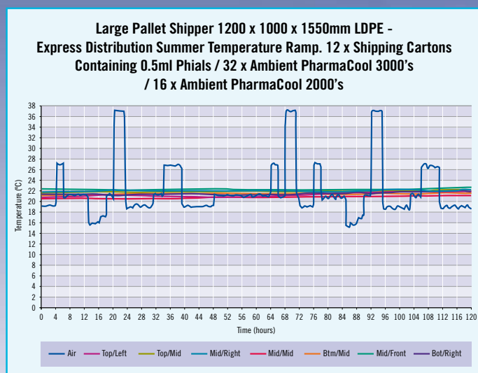
Large Pallet Shipper +15°C to +25°C
